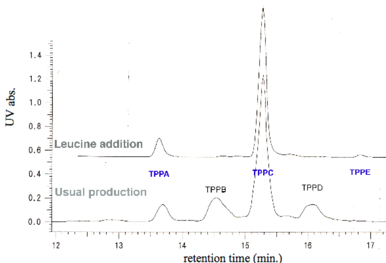
Figure 3. HPLC chromatograms (UV detection at 205 nm) of TPPs production of standard culture (lower) and 1 g/flask of L-leucine was added to the culture (upper) (for chromatographic protocol see experimental section).
