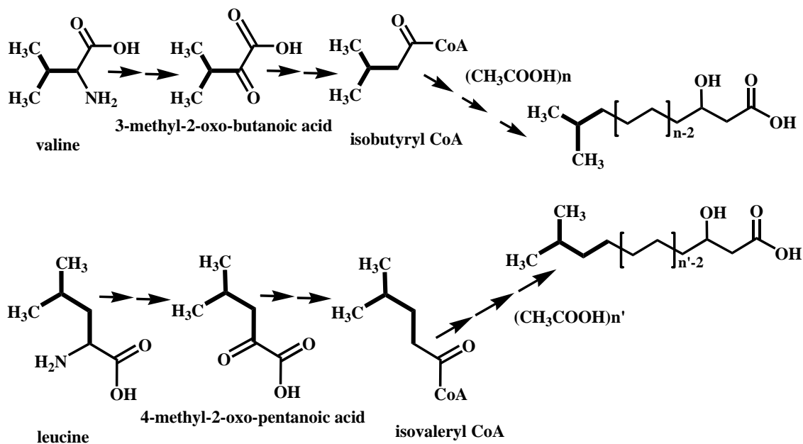
Figure 2. Branched-chain fatty acid synthetic pathway.
