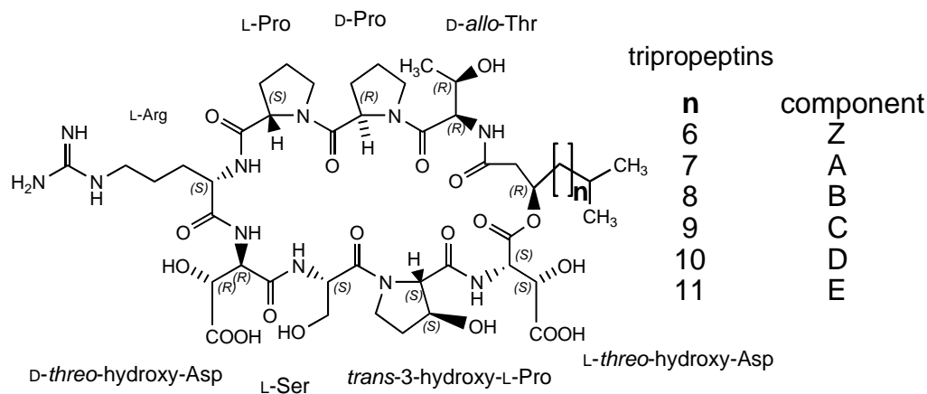
Figure 1. Structure of TPPs.
