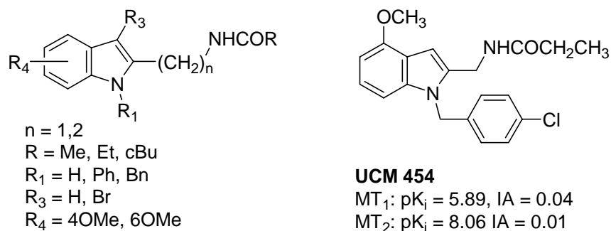
Figure 1. 2- N -Acylaminoalkylindole derivatives.
