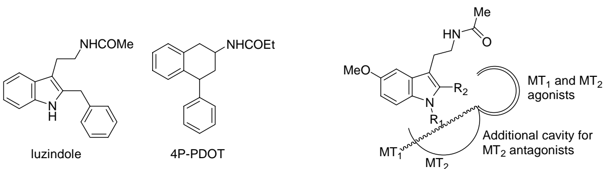
Figure 2. Left. MT 2 selective antagonists. Right. MT 1 /MT 2 selectivity: the binding site hypothesis.
