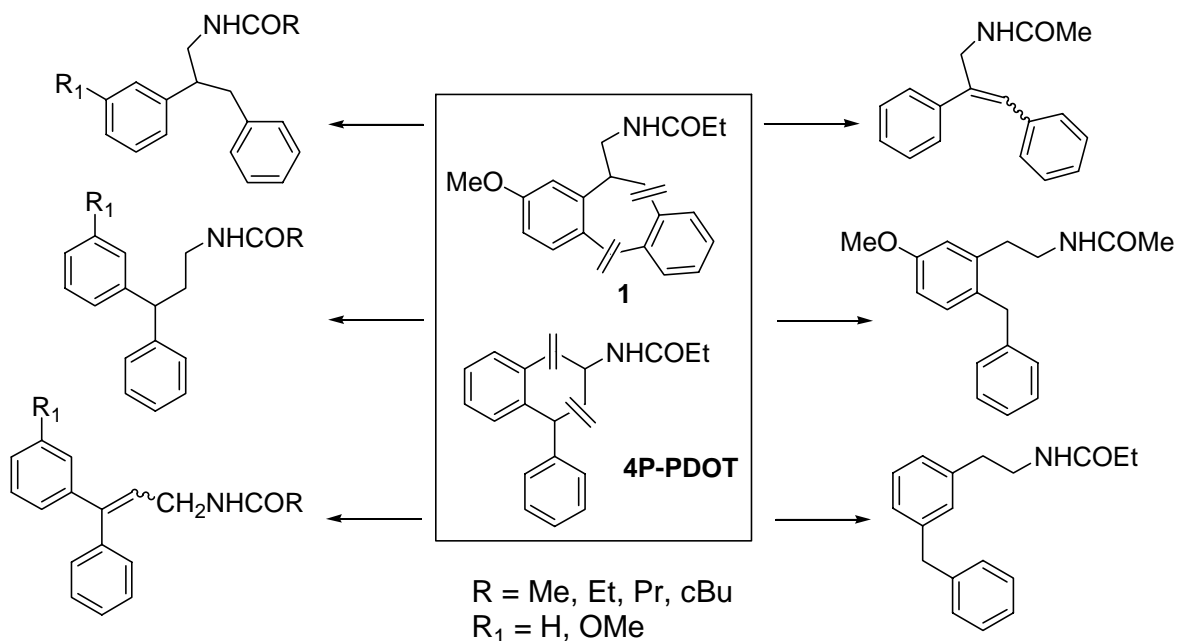
Figure 6. Non-cyclic melatonin receptor ligands.
