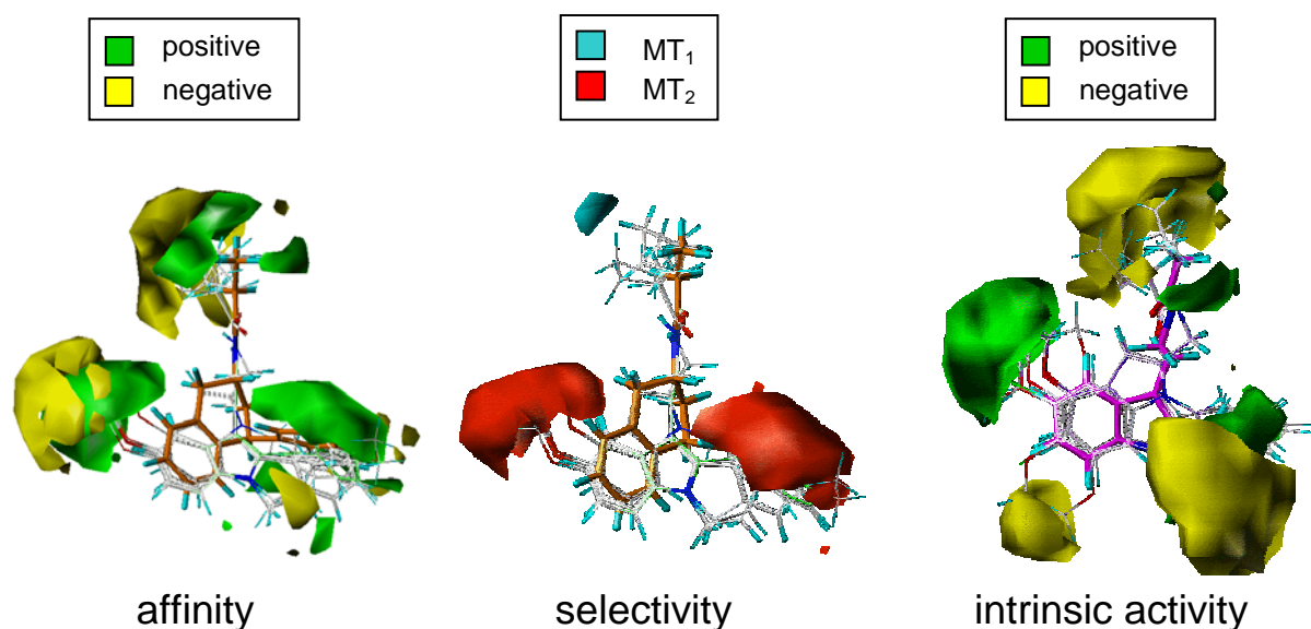
Figure 3. Left: CoMFA steric contour plots for structure-affinity analysis performed on antagonist compounds at MT 2 receptor. 4P-PDOT is depicted in capped sticks with orange carbons. Center: CoMFA steric contour plots for MT 1 /MT 2 selectivity analysis. Right: CoMFA steric contour plots for structure-intrinsic activity analysis at MT 2 receptor. Luzindole is shown in capped sticks with magenta carbons.
