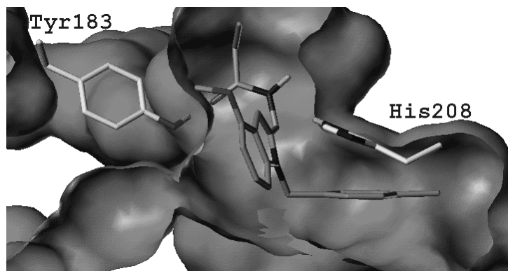
Figure 5. UCM 454 within the binding site of the MT 2 receptor model.
