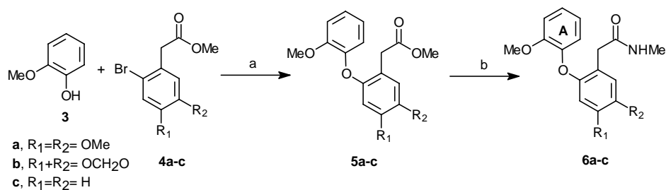
Scheme 2. (a) Cu/CuO//Py, reflux, 36h; (b) MeNH 2 /NaCN/MeOH, 60 °C, 2 h.
