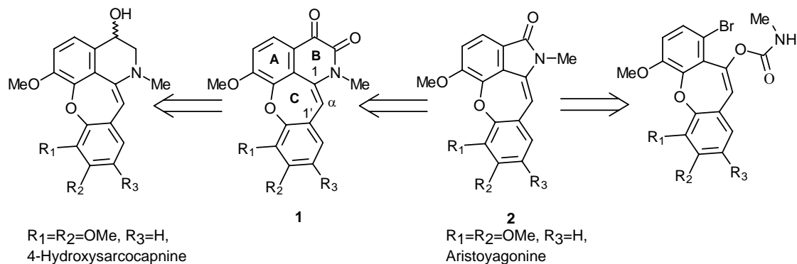
Scheme 1. Synthetic pathways to 3,4-dioxocularine and aristocularine alkaloids.
