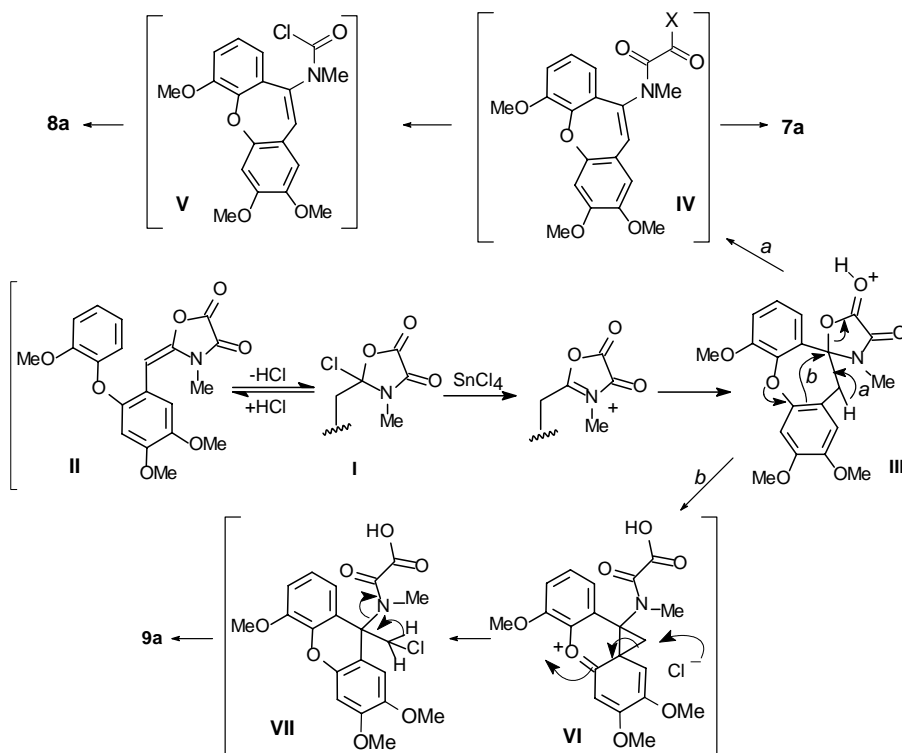
Scheme 5. Cyclization of amides with oxalyl chloride and stannyl chloride.
