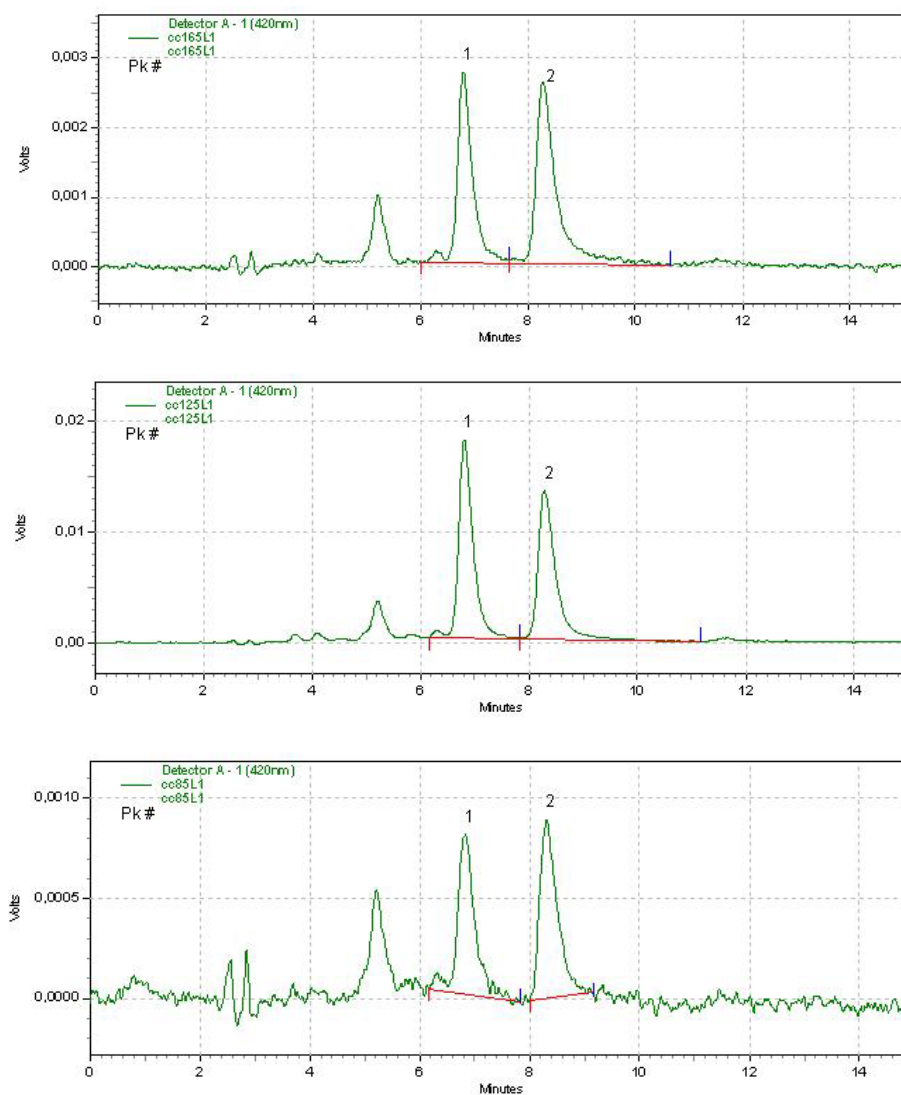
Figure 5. HPLC profile (UV detection at 420 nm) of callus extracts at early growth phase. 22 \beta -hydroxymaytenin ( 1 ) and maytenin ( 2 ). (for chromatographic protocol see experimental section).
