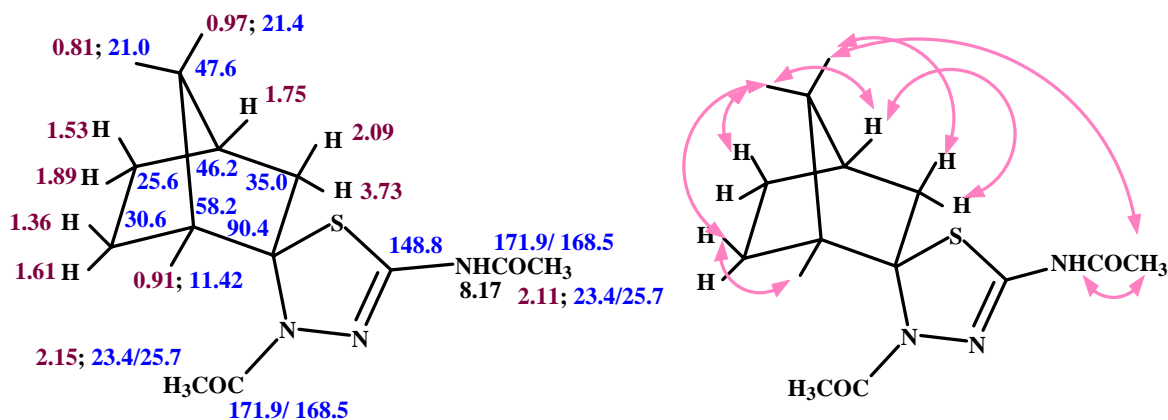
Figure 5. Spectroscopic data of 8 .
