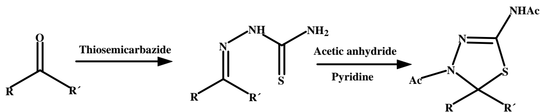
Scheme 1. General pathway for thiadiazolines's synthesis.
