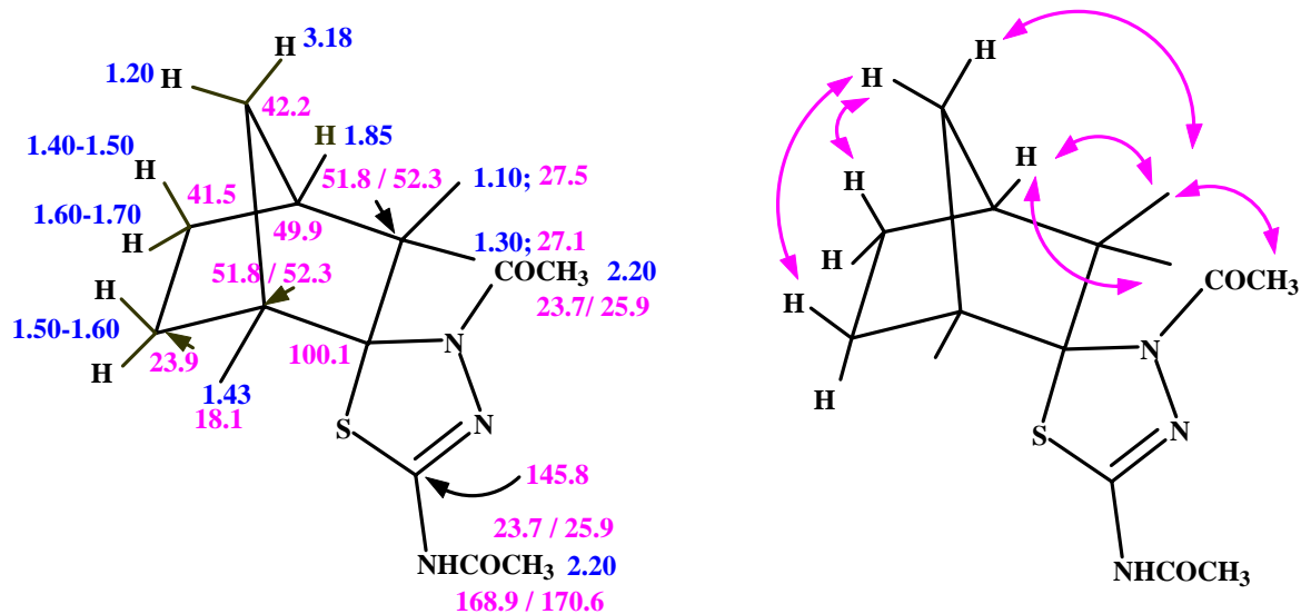
Figure 3. Spectroscopic data of 7 .
