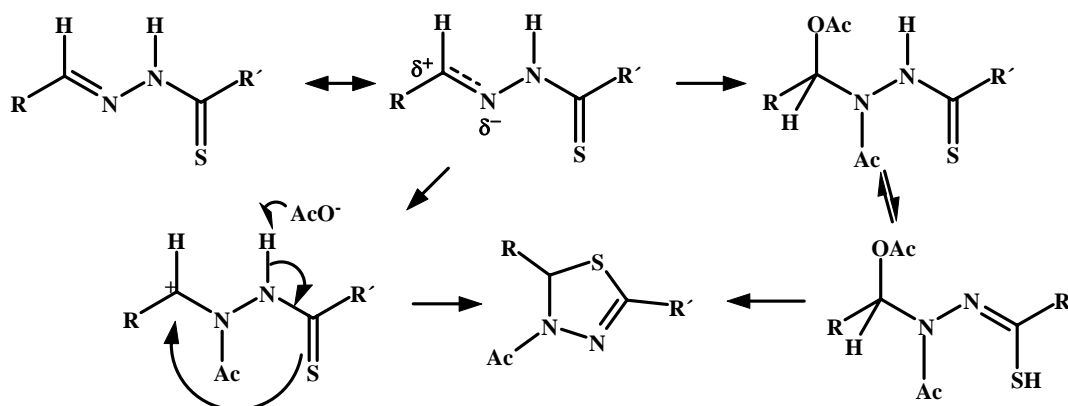
Scheme 2. Mechanism proposed for the heterocyclization reaction.
