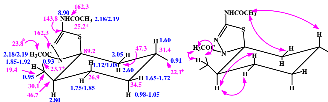
Figure 7. Spectroscopic data of 10 .
