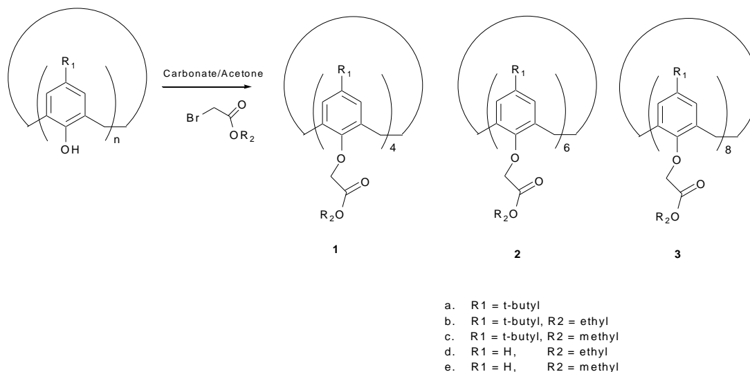
Scheme 1. Preparation of calixarene esters.
