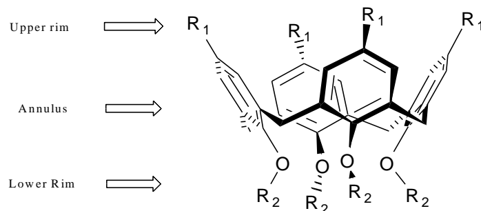
Figure 1. Cone conformation of a typical calix[4]arene.
