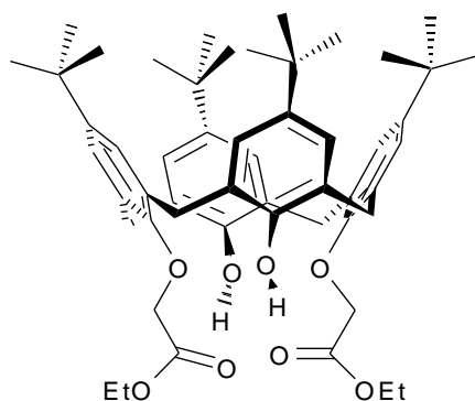
Figure 3. 1,3-disubstituted-tetra-t-butylcalix[4]arene.
