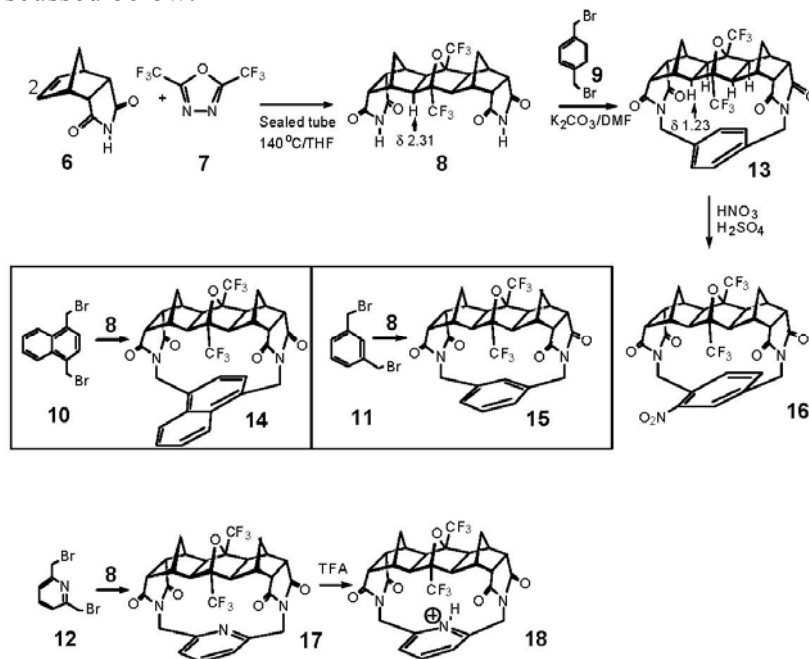
Scheme 1. Synthesis of m - and p -cyclophanes
