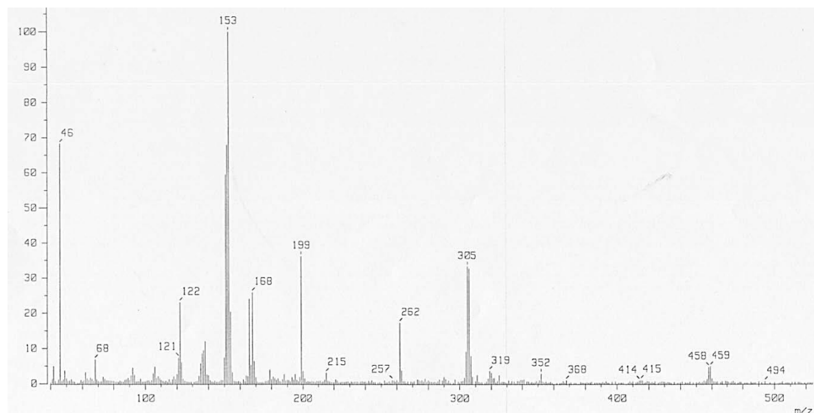
Figure 4. Negative ion FAB mass spectrum of compound 2d recorded with NBA
