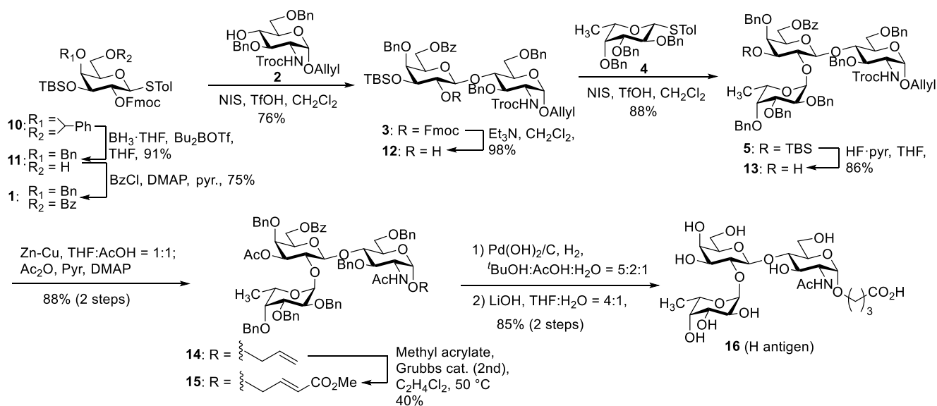
Scheme 2. Synthesis of H antigen 16
