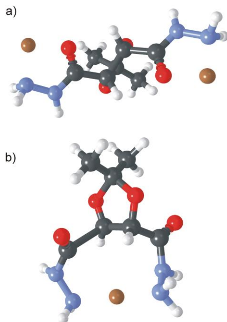
Figure 2. Complex structure of tartrate dicarbohydrazide 2 with a) two ( \text{M}_2\text{L} ) and b) one ( \text{ML} ) \text{Cu}^{2+} ion(s) calculated by PM6 method (MOPAC 2009).
