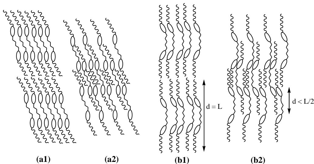
Figure 1. Schematic representations of mesophases. (a1) Single layer and (a2) intercalated untilted smectic A phases composed of even-membered dimers. (b1) Single layer, layer spacing equals the molecular length L and (b2) intercalated tilted anticlinic smectic C_A phases composed of odd-membered dimers.
