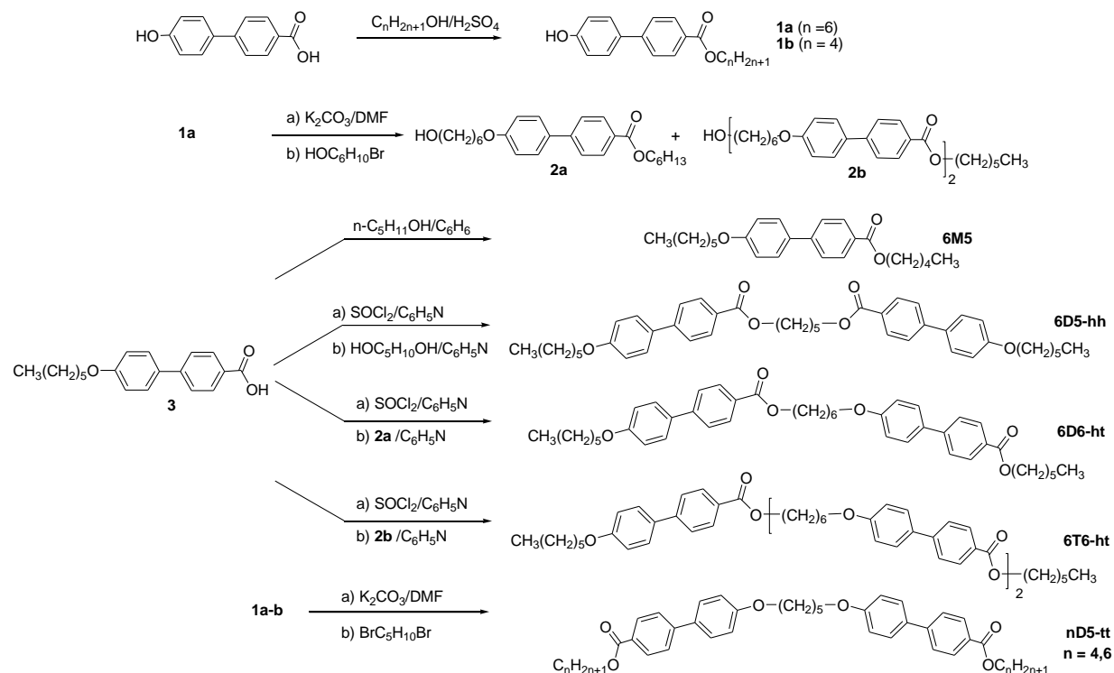
Scheme 1. Synthesis of the alkoxybiphenylcarboxylic esters.
