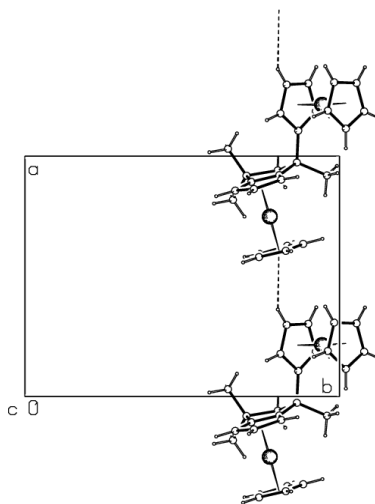
Figure 2. A crystal packing diagram of 4 , viewed along the c axis, showing the C–H \cdots \pi interaction which links the molecules into infinite chains. The C–H \cdots \pi interaction is indicated by dotted lines.
