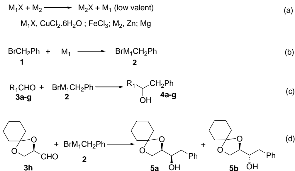
Scheme 1. Low valent metal mediated benzylation of aldehydes.
