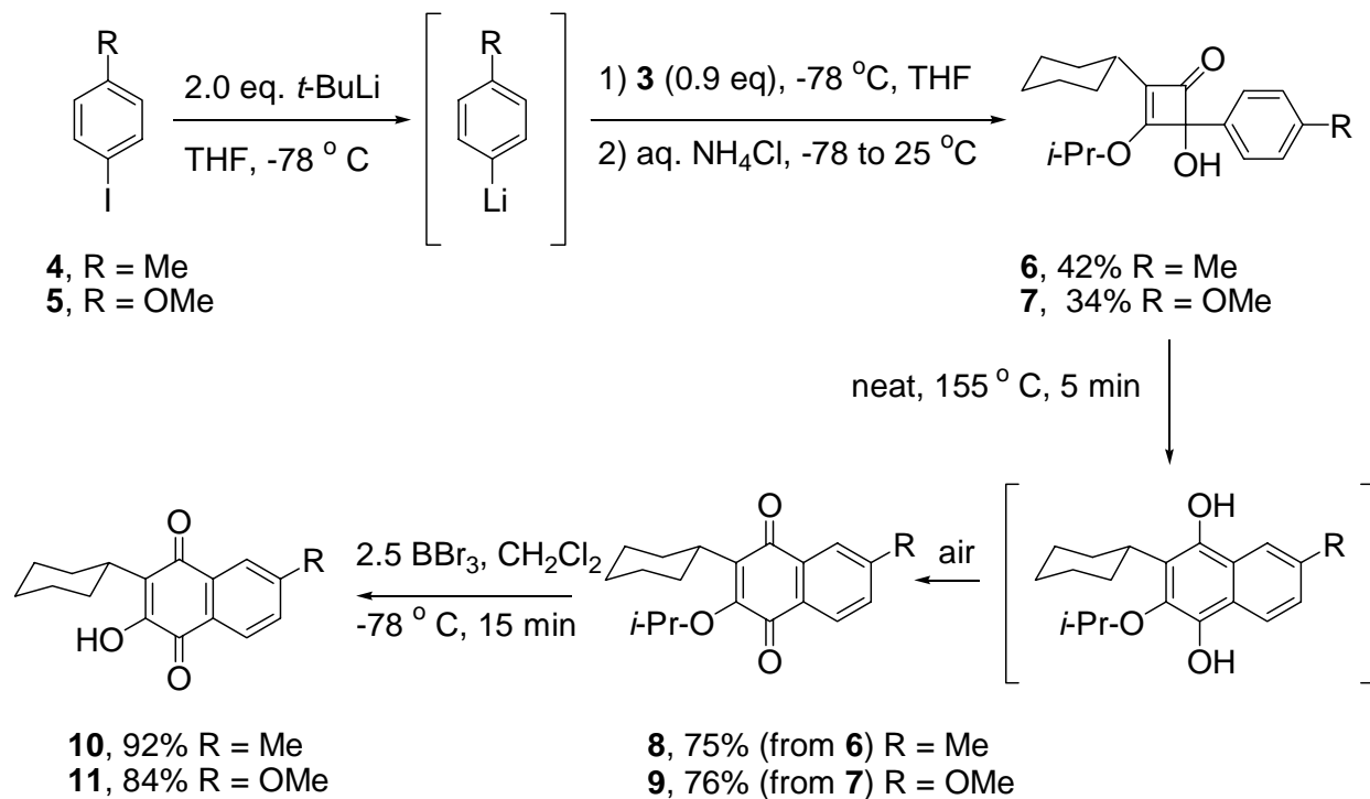
Scheme 1. Completion of the synthesis of parvaquone analogues 10 and 11 .
