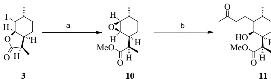
Scheme 6. a. \text{Na}_2\text{CO}_3 , \text{CH}_3\text{OH} , reflux, 72%. b. \text{Cp}_2\text{TiCl} , Zn, \text{ZnCl}_2 , THF, 0^\circ\text{C} , 10%.
